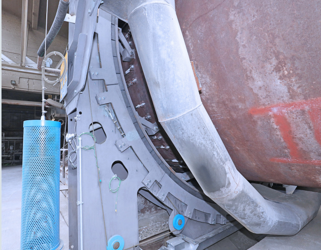
Two separate tensioning ropes for the upper and lower strand ensure easy and uniform pretensioning by steel weights.
